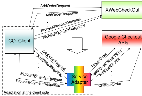
Figure 2: CO_Client to replace XWebCehckout service with Google checkout APIs using adapters
