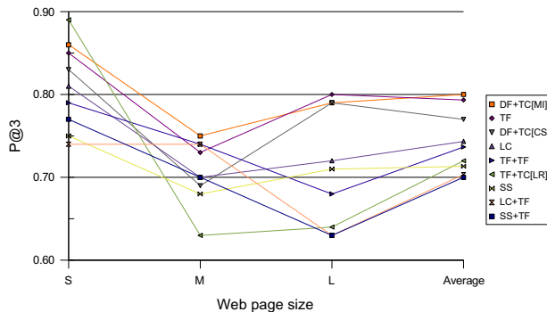
Figure 1: Precision at the first three output annotations for the best methods of each category.
